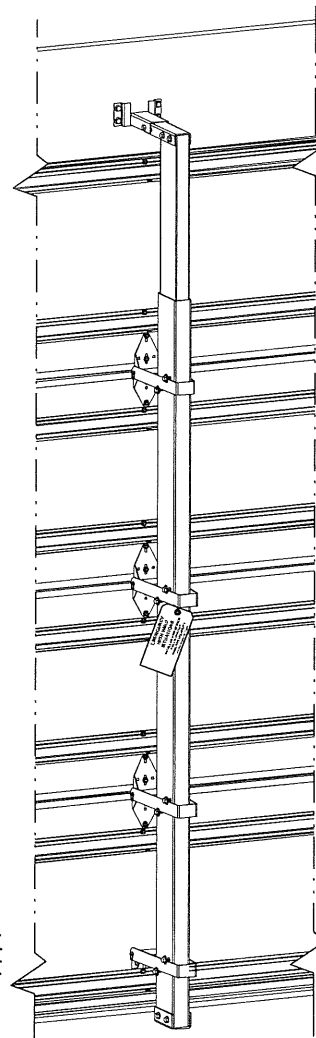
COMPLETED INSTALLATION ON (4) SECTION DOOR
